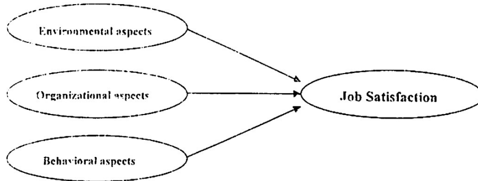
Fig 1: Research Model
